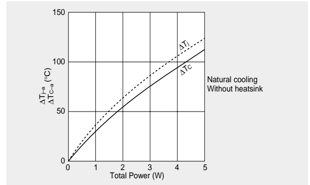
Fig. 8 Temperature rise
